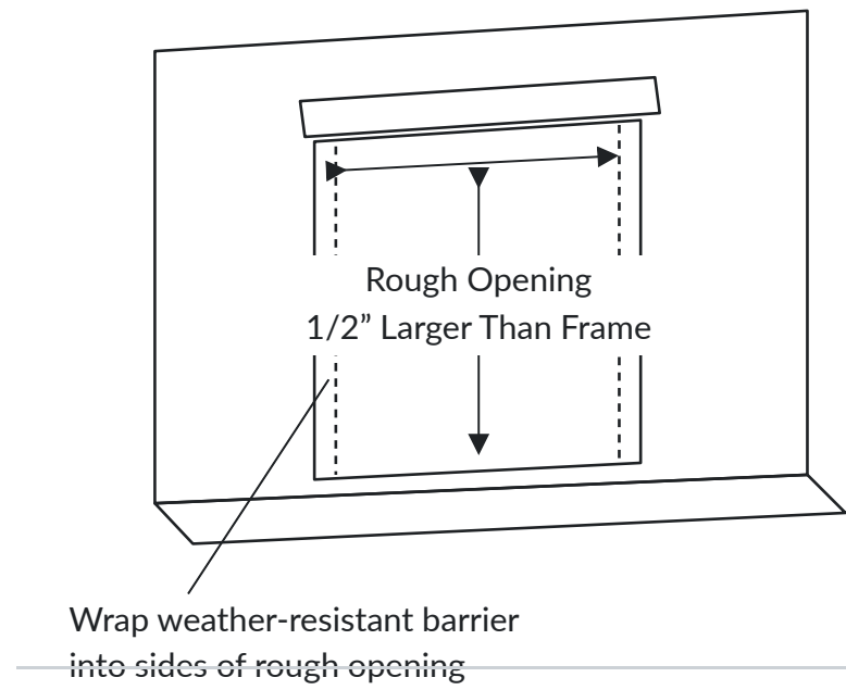
ROYAL WINDOOR · Experience Excellence Figure 3 — Typical Rough Opening
